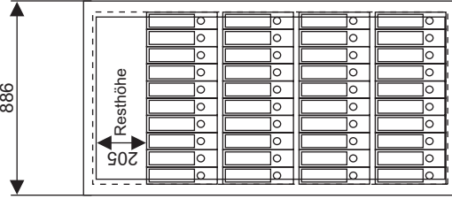
Art. 43102-43103 40 Ordner 75mm (4 Reihen)
