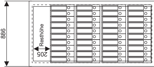
Art. 44602-44603 40 Ordner 75mm (4 Reihen)
